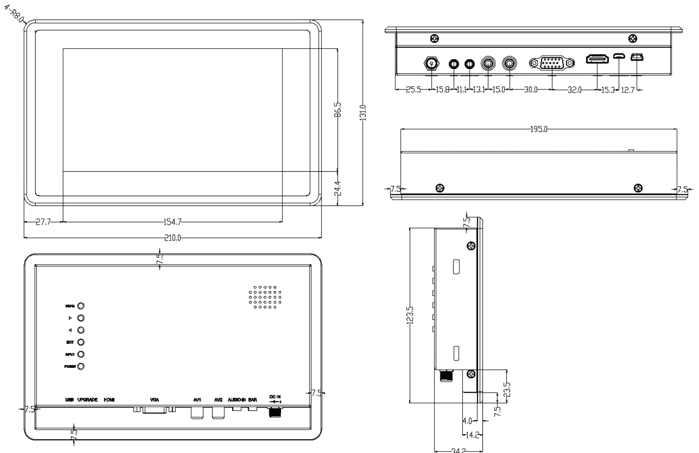
Structure Diagram (Mounting Hole Size: 197 x 119 mm)
